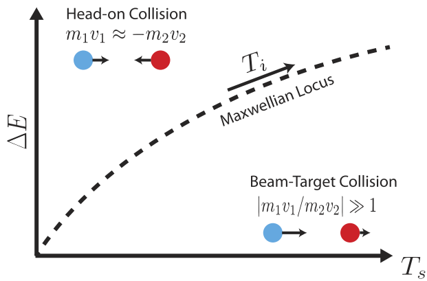
Figure 2. Diagram of the (\Delta E, T_s) spectral moment space. Collisions of high K and low v_{\text{cm}}^2 produce spectra with moments in the upper left. Collisions of low K and high v_{\text{cm}}^2 lie in the lower right—assuming that the distribution of \vec{v}_{\text{cm}} is isotropic. Also shown is the Maxwellian locus which gives a 1-to-1 relationship between \Delta E and T_s . Changing the thermodynamic temperature simply moves one along this locus and the rest of the space remains inaccessible.
