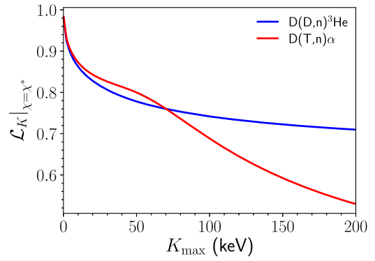
Figure 6. The momenta-matched relative kinetic energy scaling as a function of K_{\text{max}} for \text{D}(\text{D}, \text{n})^3\text{He} and \text{D}(\text{T}, \text{n})\alpha . It can be seen that the resonance in the DT cross section at \sim 60 keV has a strong effect on the relative kinetic energy.
